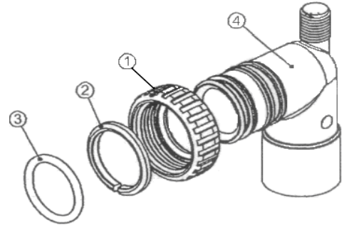
3/4" & 1" PVC SOLVENT ELBOW
