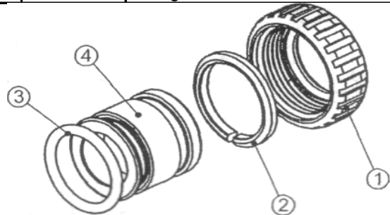
3/4" BRASS SWEAT
