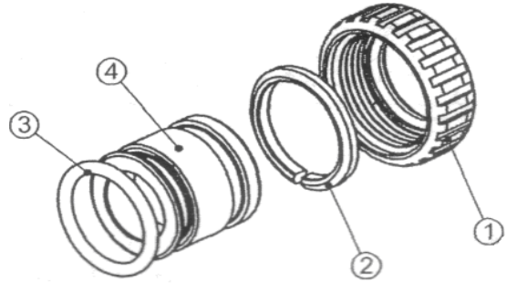
3/4" BRASS SWEAT
