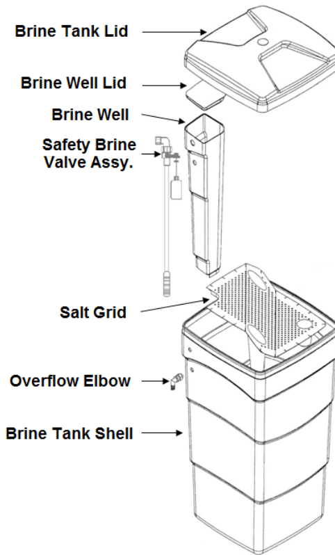
FIGURE 7: Brine Tank
