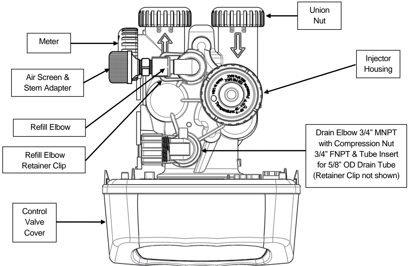
FIGURE 6: Top View of Control Valve
