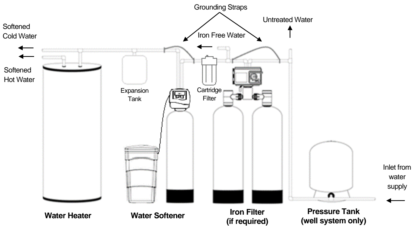
FIGURE 1: Typical Installation
