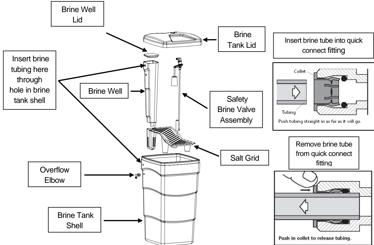
FIGURE 3: Brine Tank Components
